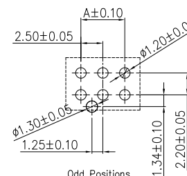
Odd Positions 2x3P.2x5P.2x7P P.C.B LAYOUT
