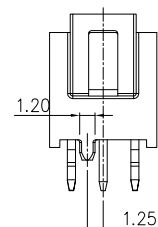
Odd Positions 2x3P.2x5P.2x7P
