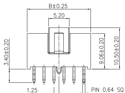
Even Positions 2x2P.2x4P.2x6P.2x8P
