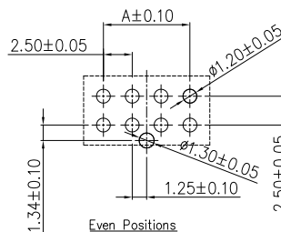
Even Positions 2x2P.2x4P.2x6P.2x8P P.C.B LAYOUT
