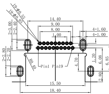
RECOMMENDED PCB LAYOUT (TOP VIEW) TOLERANCE: ±0.05mm
