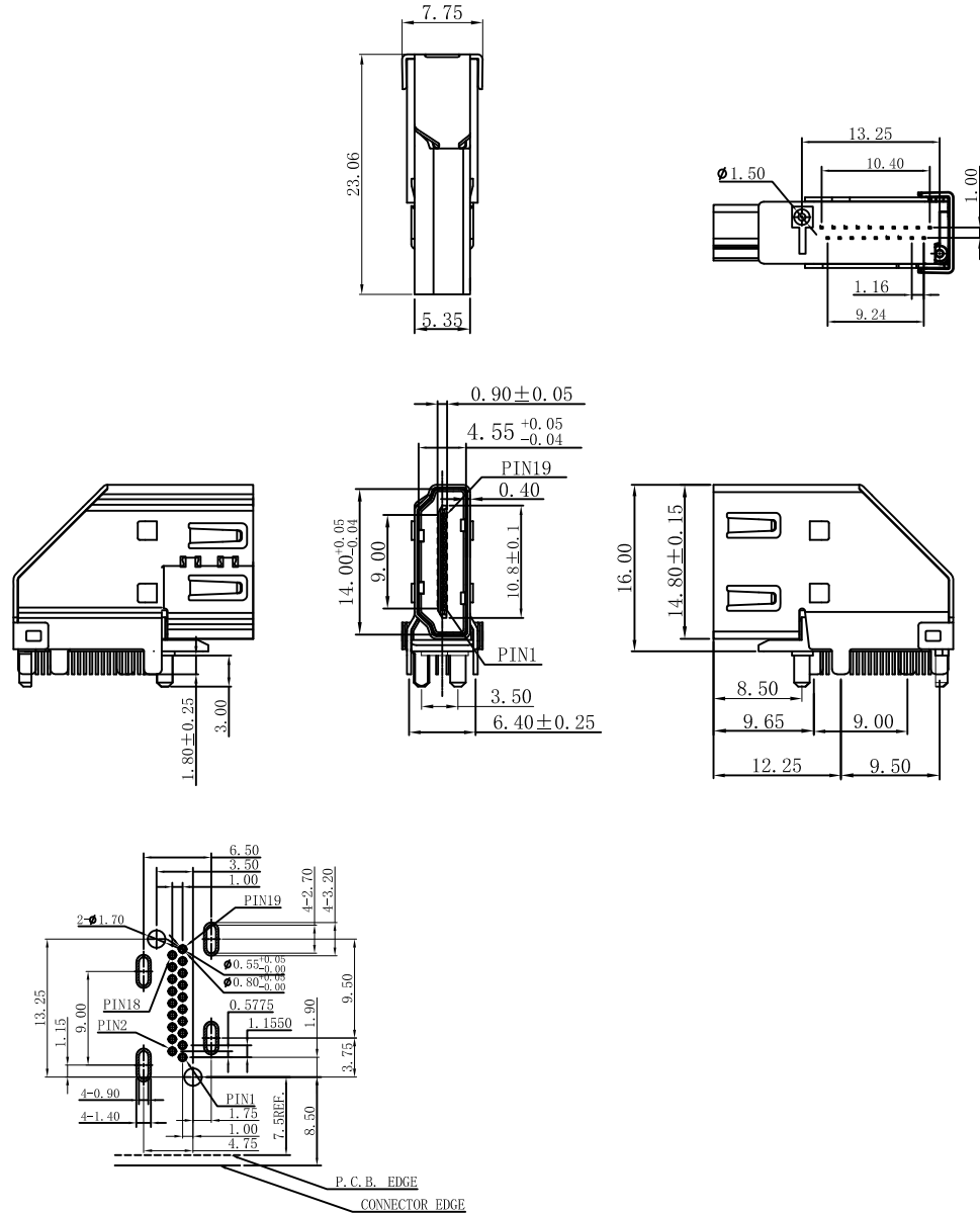
RECOMMENDED PCB LAYOUT (TOP VIEW) TOLERANCE: ±0.05mm
